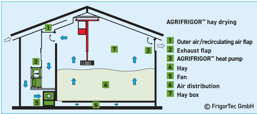
11 AGRIFRIGOR™ process of drying hay by heat pump or dehumidifier
