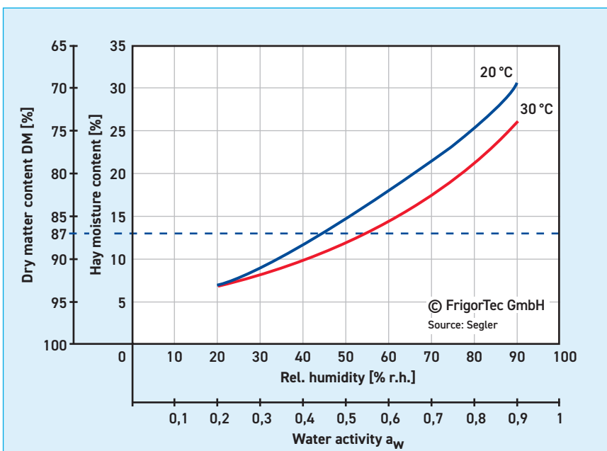
21 Sorption isotherms of hay
