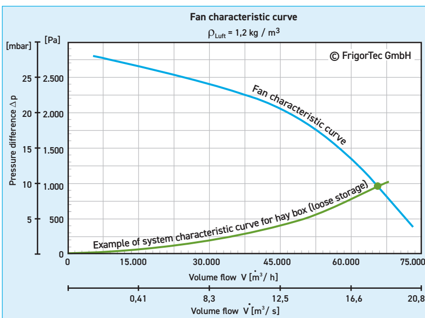
20 Characteristic curve of an AGRIFRIGOR™ fan
