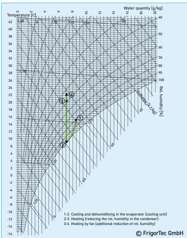
13 Heat pump process in Mollier-h-x diagram
