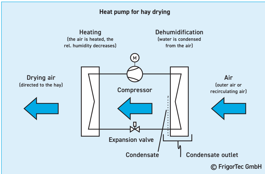
12 Heat pump process for air dehumidification
