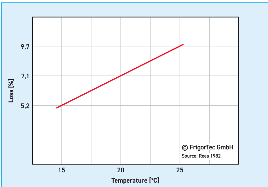
26 Respiration losses in field drying
