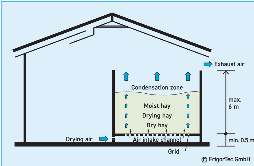
25 Drying process in the hay box
