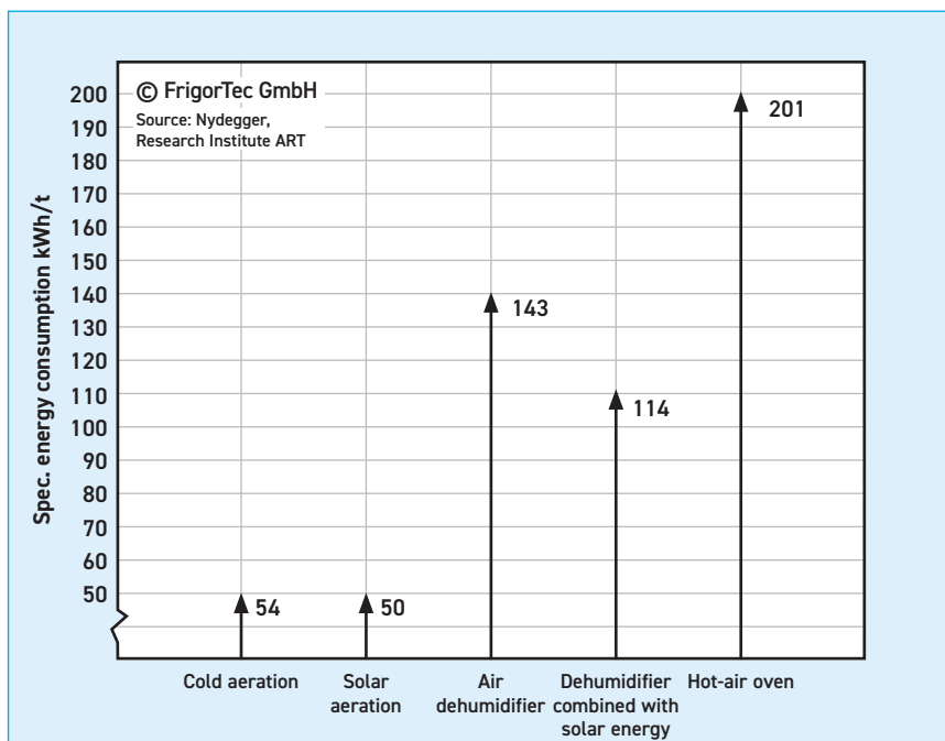
29 Specific energy consumption of various hay drying methods (17)
