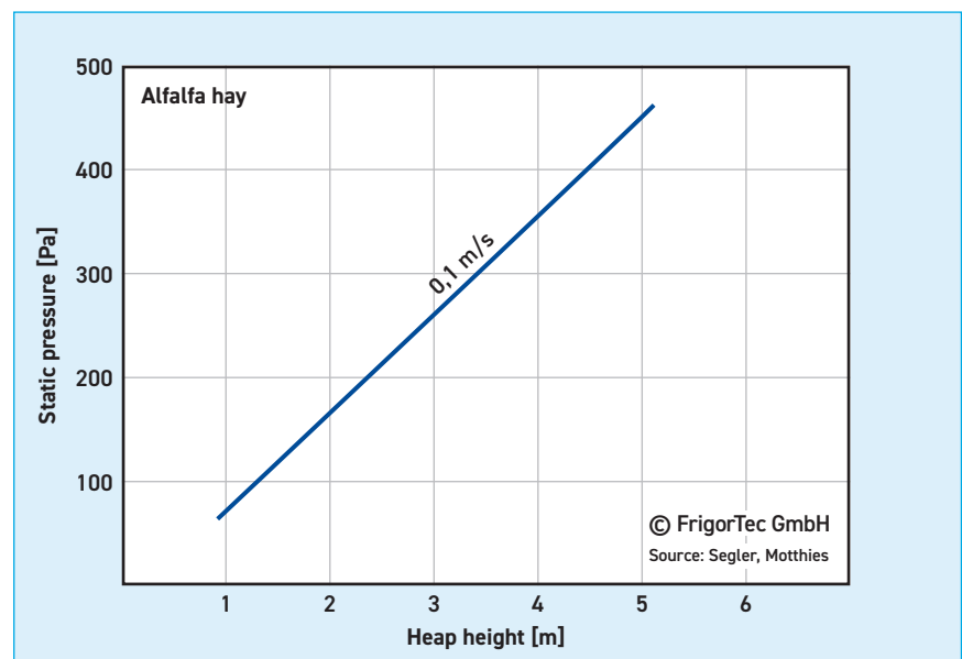
18 Pressure loss with alfalfa hay (6)
