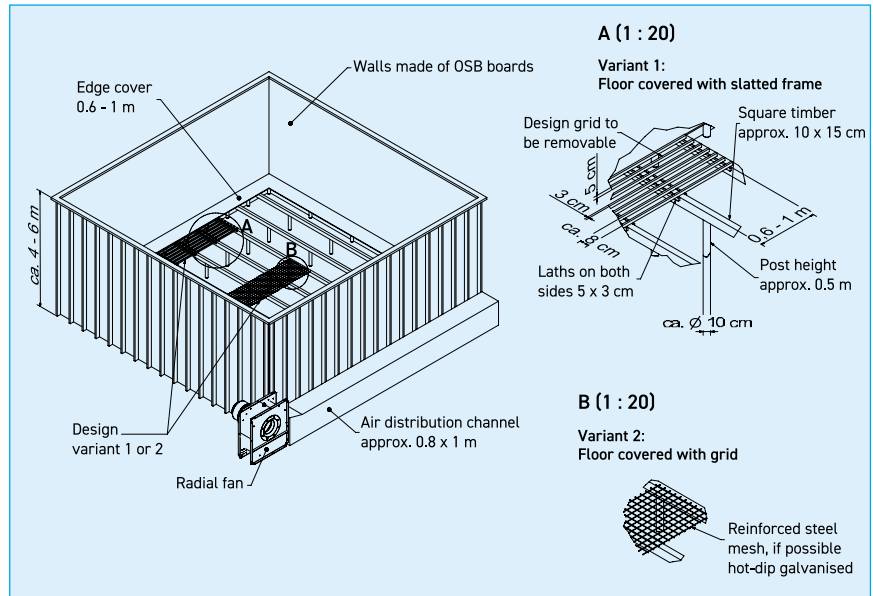
22 Design drawing of hay box with slats/grid
