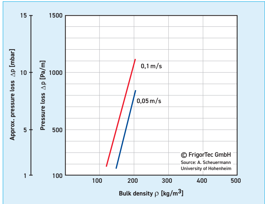
28 Pressure loss of meadow hay with high leaf content (13)
